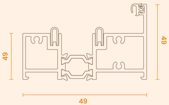
Upstand Track
