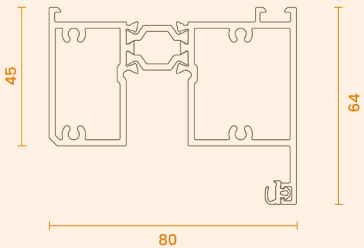
Top Track
